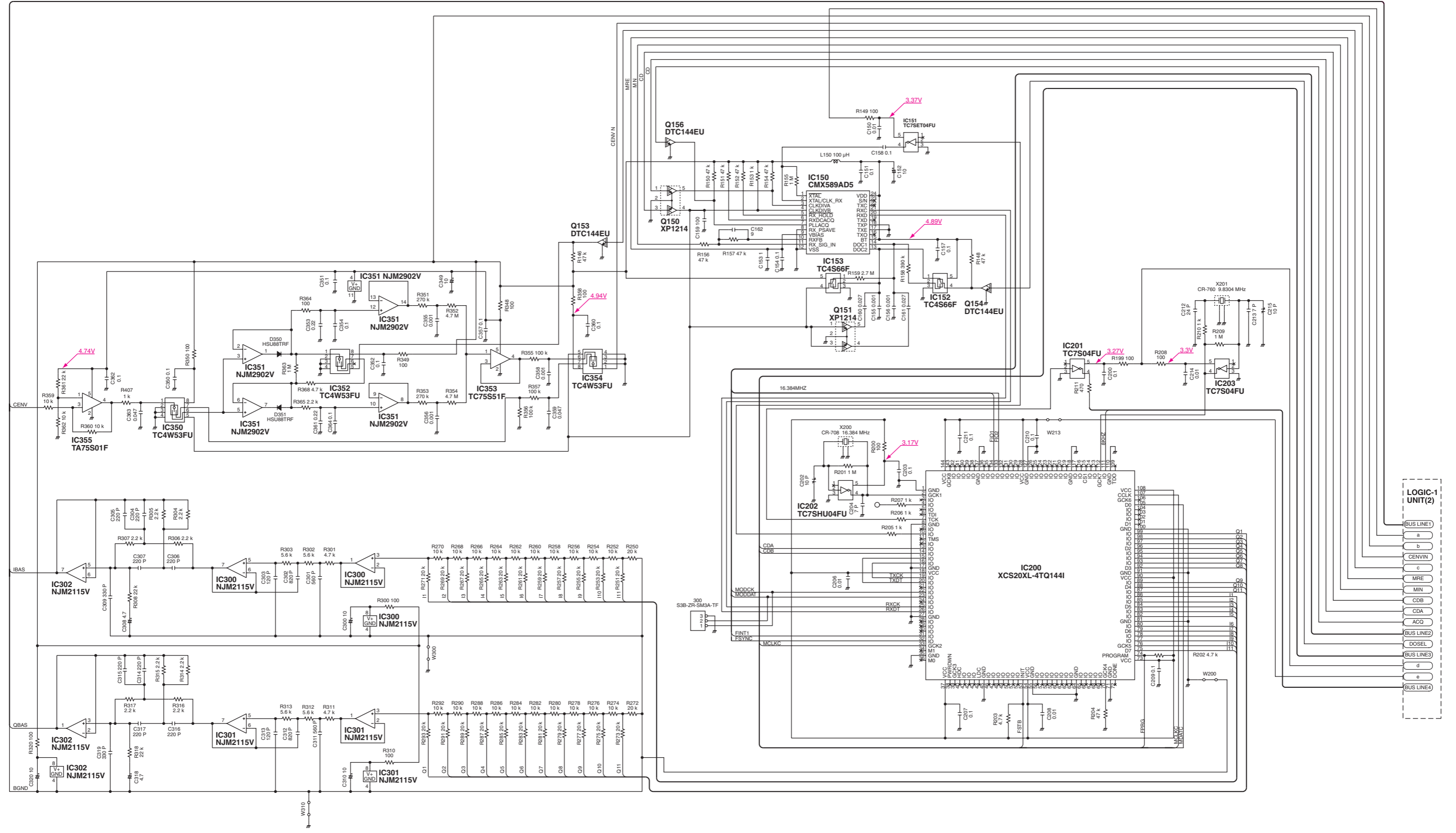
LOGIC-1 UNIT(1)
